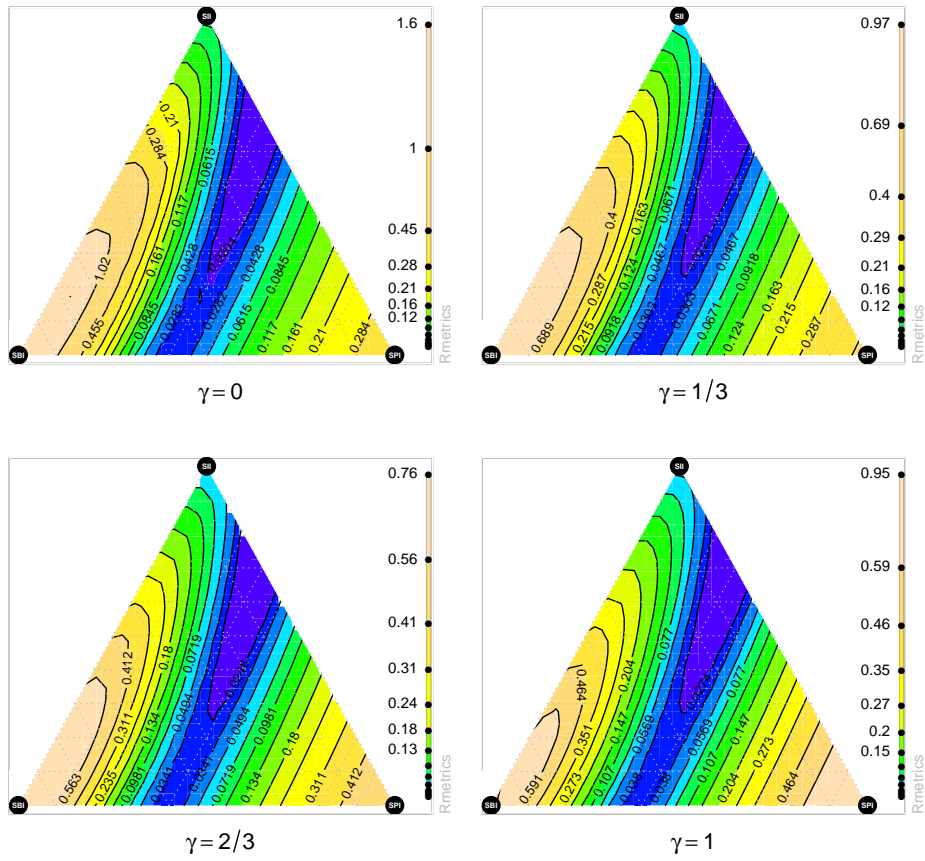
Figure 7: Ternary plot to illustrate the shape of the divergence measure for the phi-portfolio with three assets portfolio with different \gamma values.
